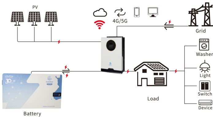
Home Energy Storage System
