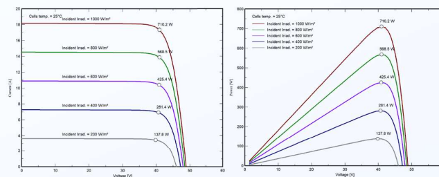
Current-Voltage Characteristic
