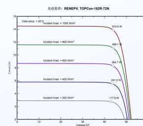
Power-Voltage Characteristic
