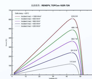
Current-Voltage Characteristic
